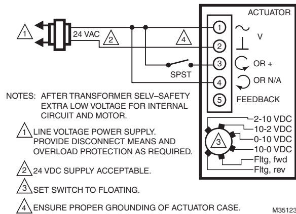
Fig. 16. Wiring for SPST on/off control.
