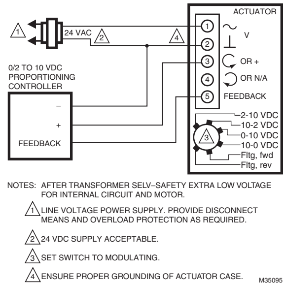
Fig. 19. Wiring for 0/2-10 Vdc modulating controllers.
