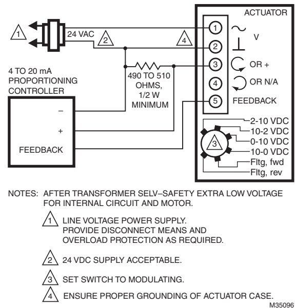
Fig. 20. Wiring for 4-20 mA modulating controllers.
