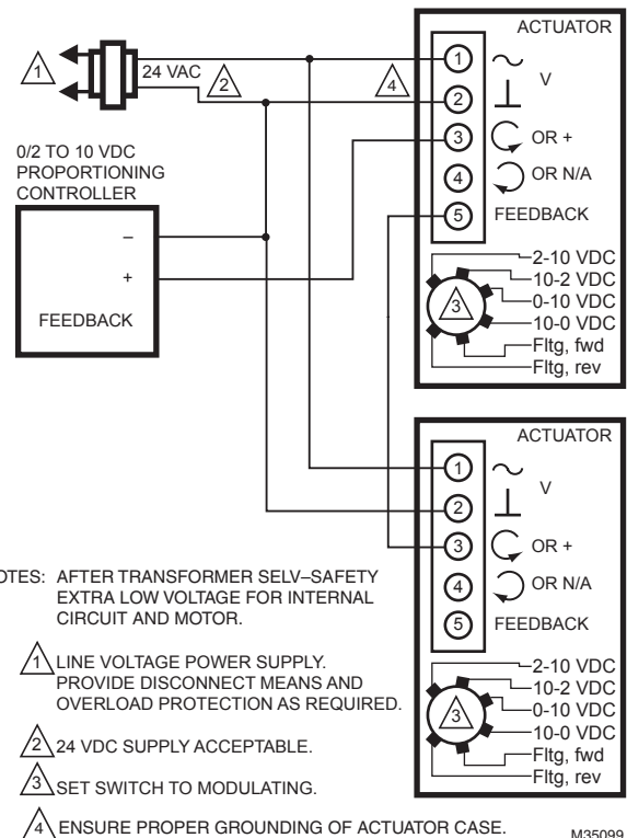
Fig. 27. Wiring for 0/2-10 Vdc modulating controller operating multiple actuators as master/drone.
