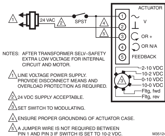
Fig. 17. Wiring for two-wire SPST on/off control.
