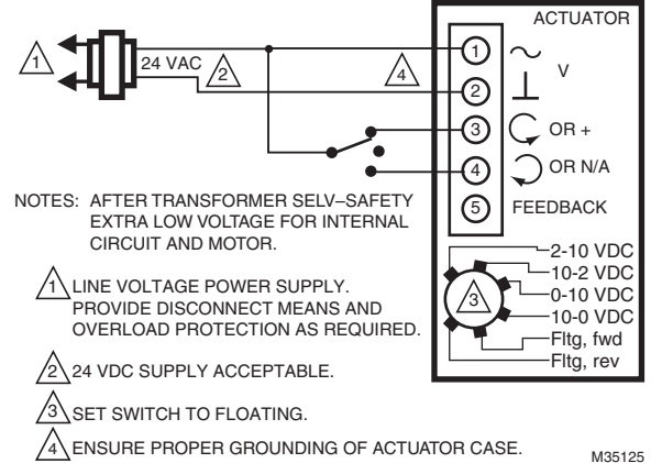
Fig. 18. Wiring for floating control.
