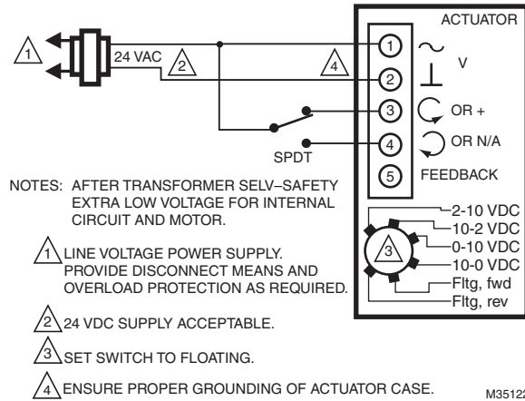
Fig. 15. Wiring for SPDT on/off control.
